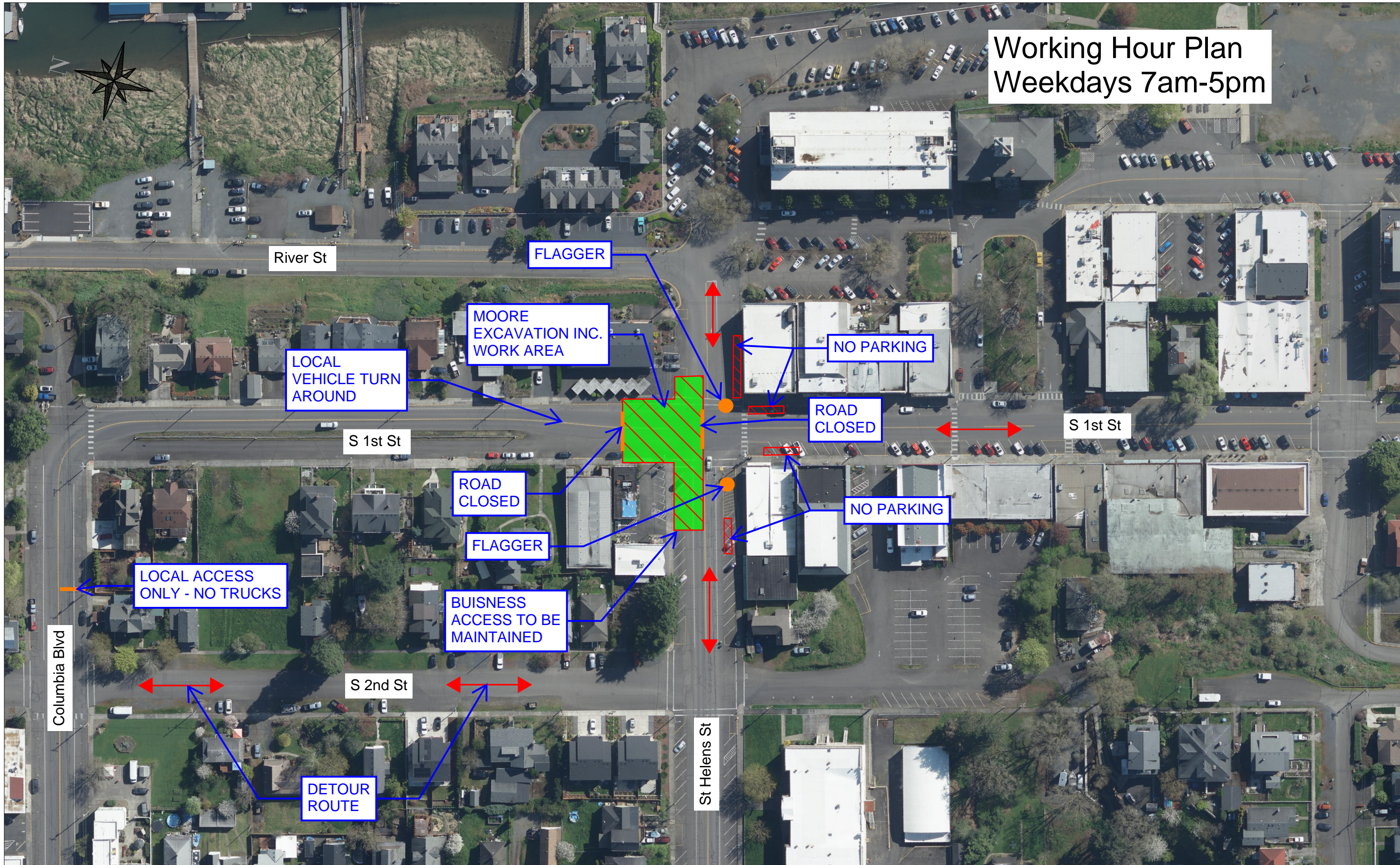
PLAN VIEW SCALE: HORZ. 1" = 100'
